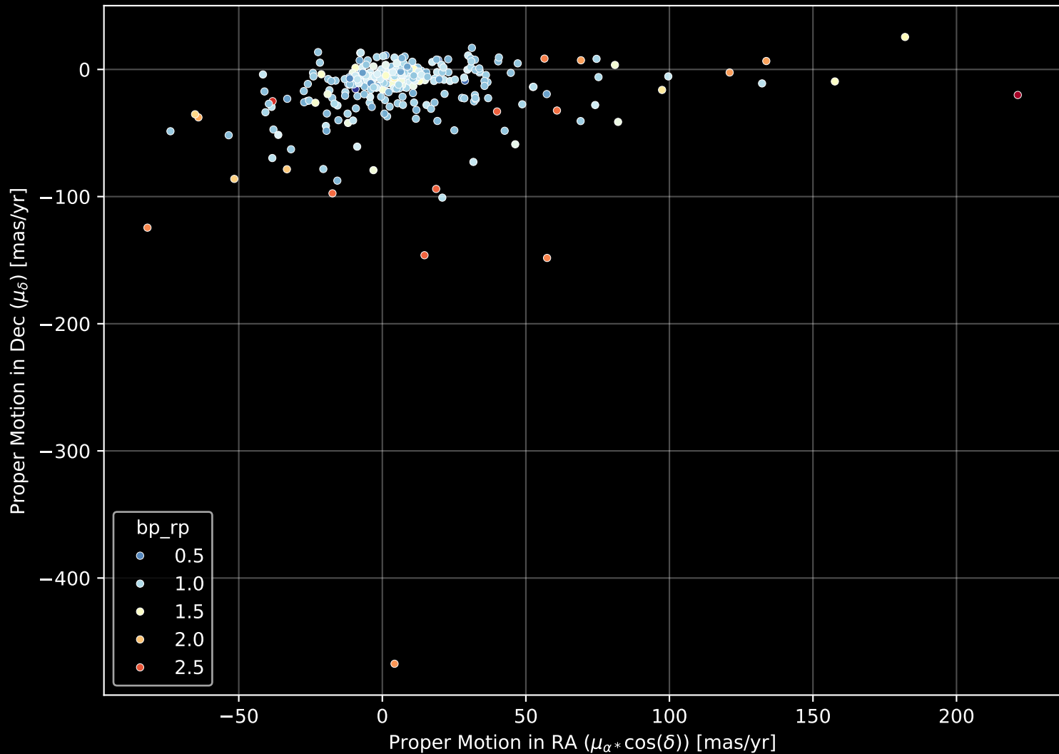
APOGEE DR17 Field: [093-43_MGA] Proper Motion Diagram (n= 294)
