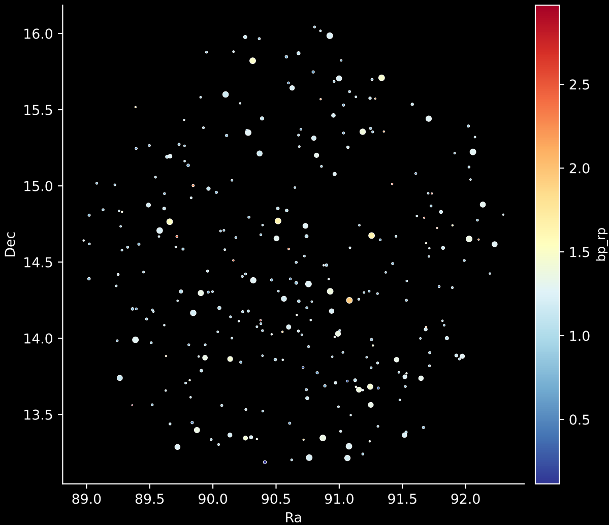
APOGEE DR17 Field: [093-43_MGA] Stars: 294
