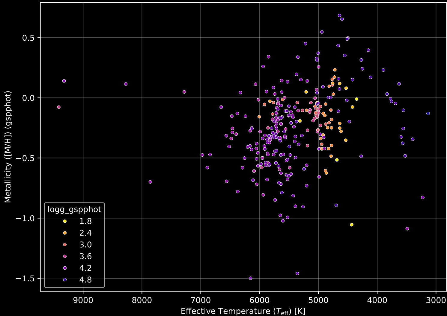
APOGEE DR17 Field: [093-43_MGA] Stellar Population Parameters (n= 294)
