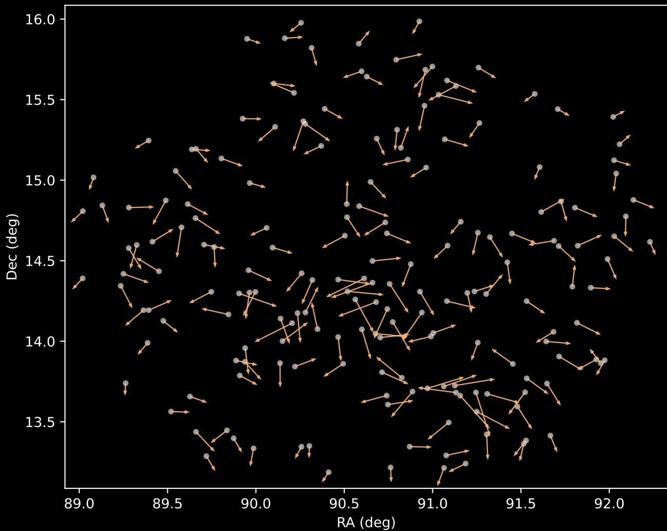
APOGEE DR17 Cluster 3 Proper Motion Vectors (n=185)
