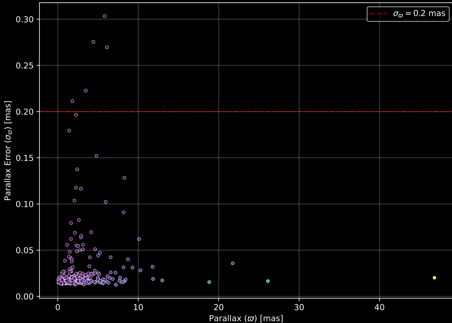
APOGEE DR17 Field: [093-43_MGA] Parallax Quality (n= 294)
