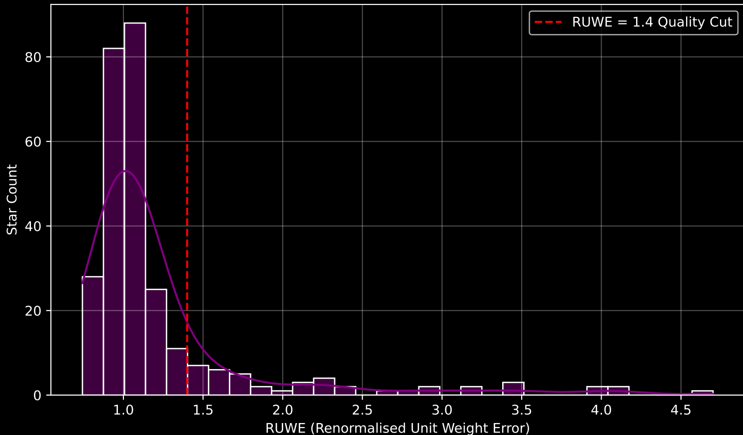
GAPOGEE DR17 Field [093-43_MGA] RUWE Distribution (n= 278)
