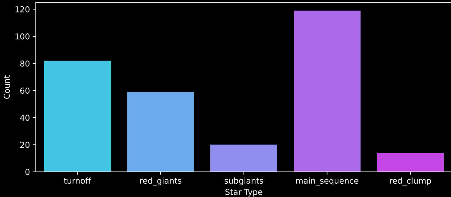
APOGEE DR17 Field: [093-43_MGA] Count plot of Star Type
