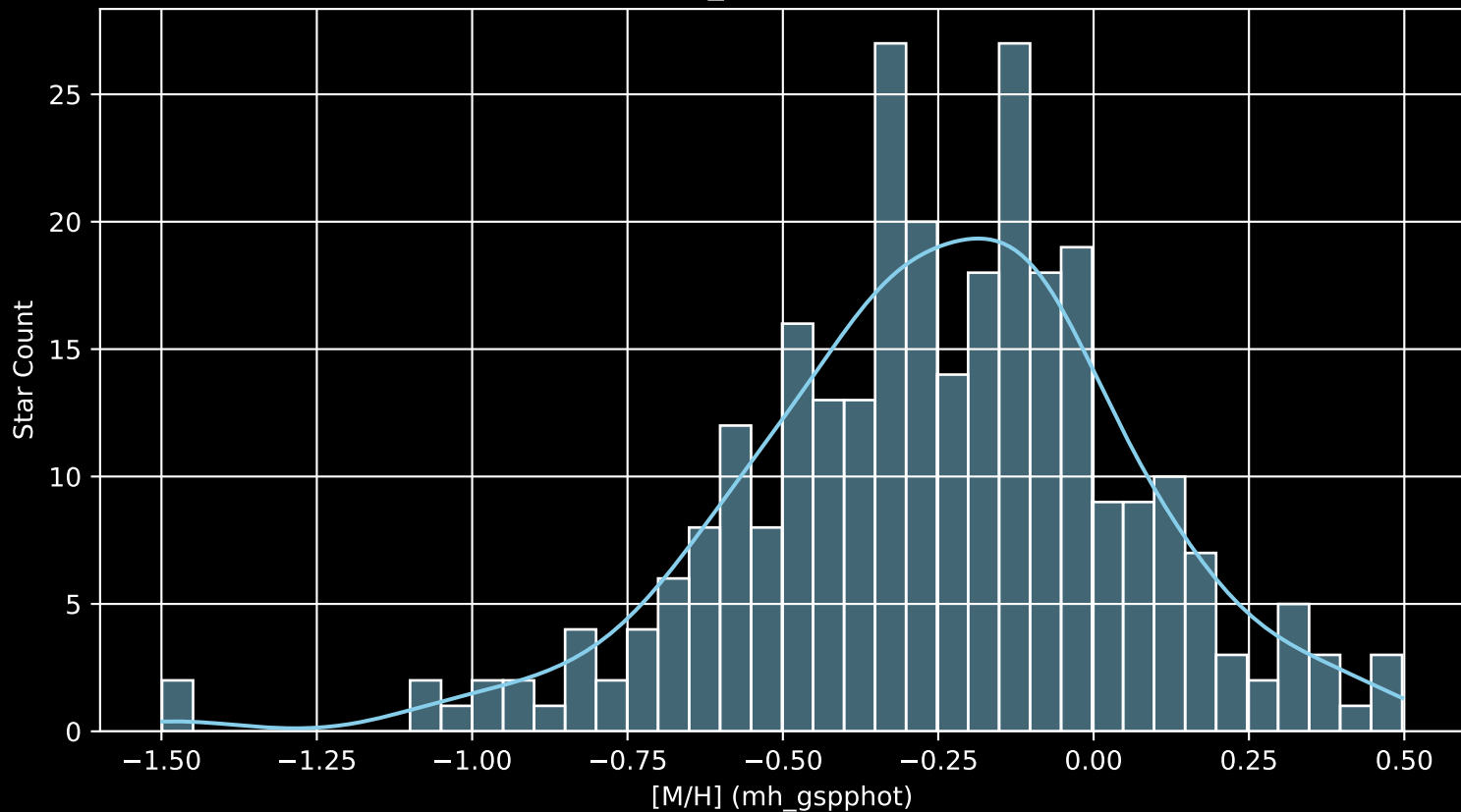
APOGEE DR17 Field: [093-43_MGA [M/H] (mh_gspphot) (n= 291)
